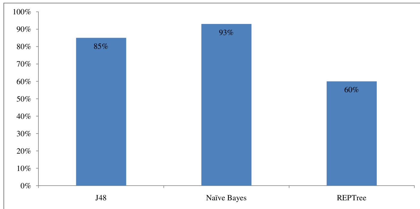
Figure-9: Comparison of Classifiers Output.
