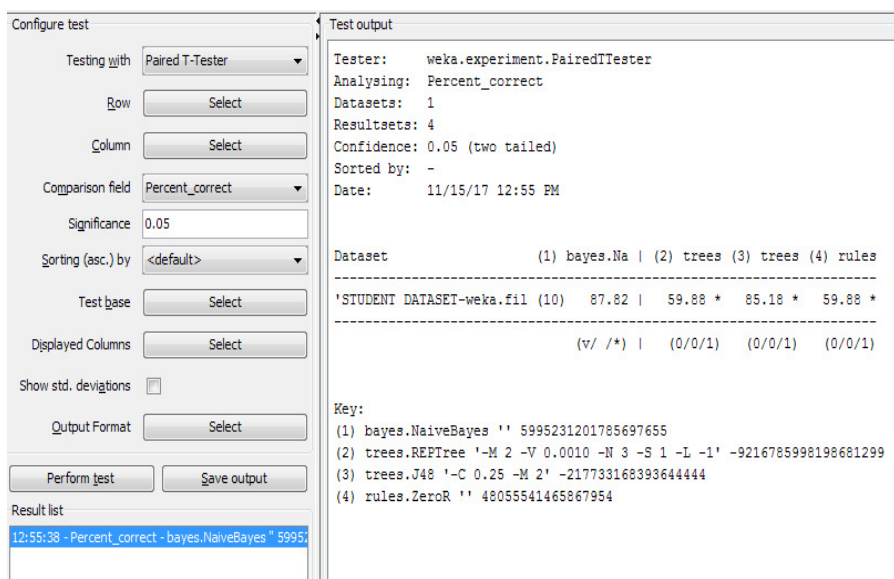
Figure-3: Comparison of Classifiers Test Output.
