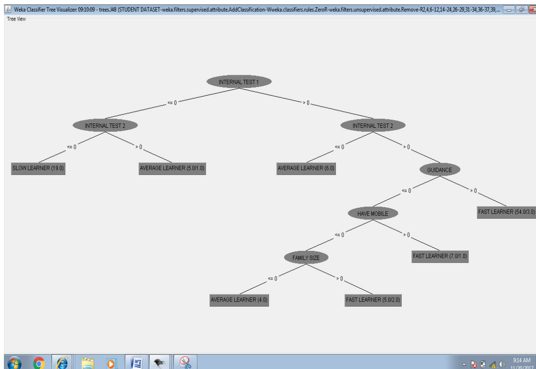
Figure-6: Decision Tree generated through J48 Classifier.
