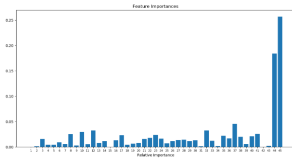
Fig.2. Feature Importance
